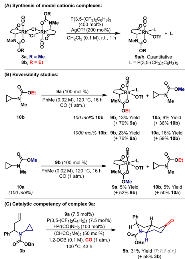
Scheme 4. Preliminary Mechanistic Studies
